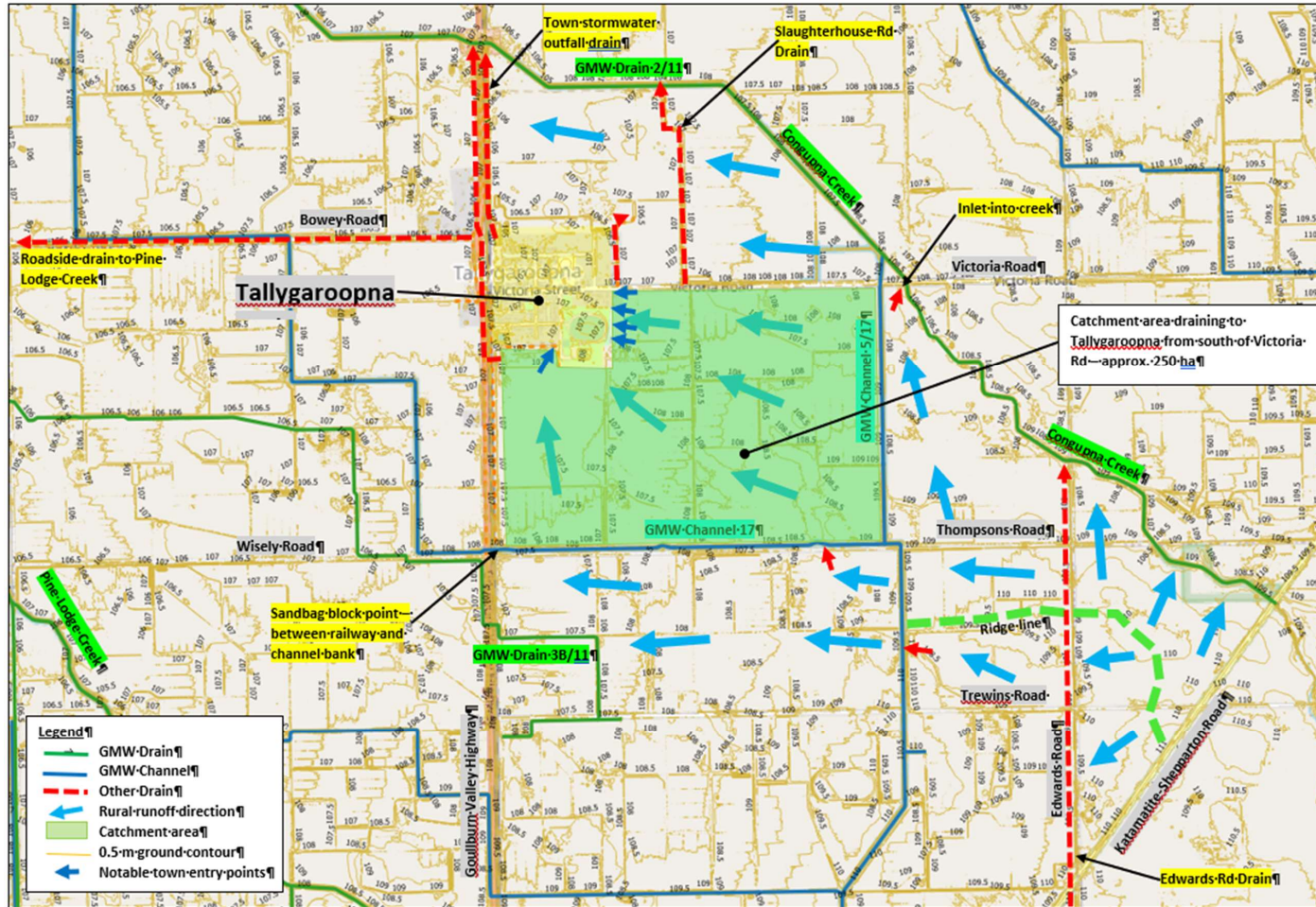
Figure 13 Tallygaroopna Township Catchment Plan
