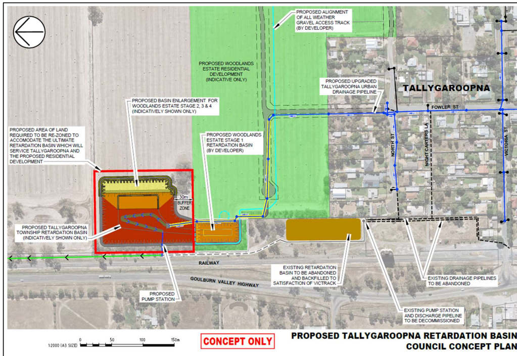
Figure 10 2021 Concept Plan for Township Stormwater Upgrades
