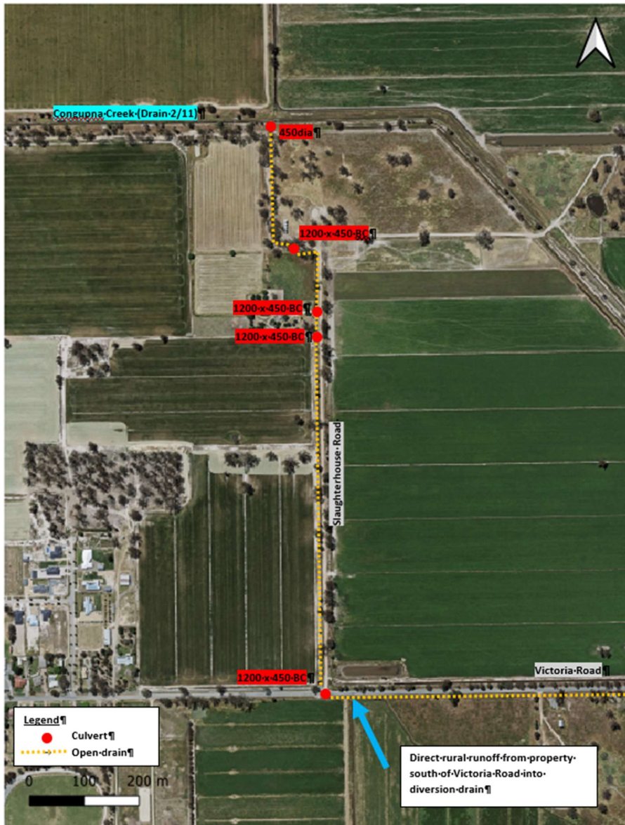
Figure 17 Slaughterhouse Road Diversion Drain
