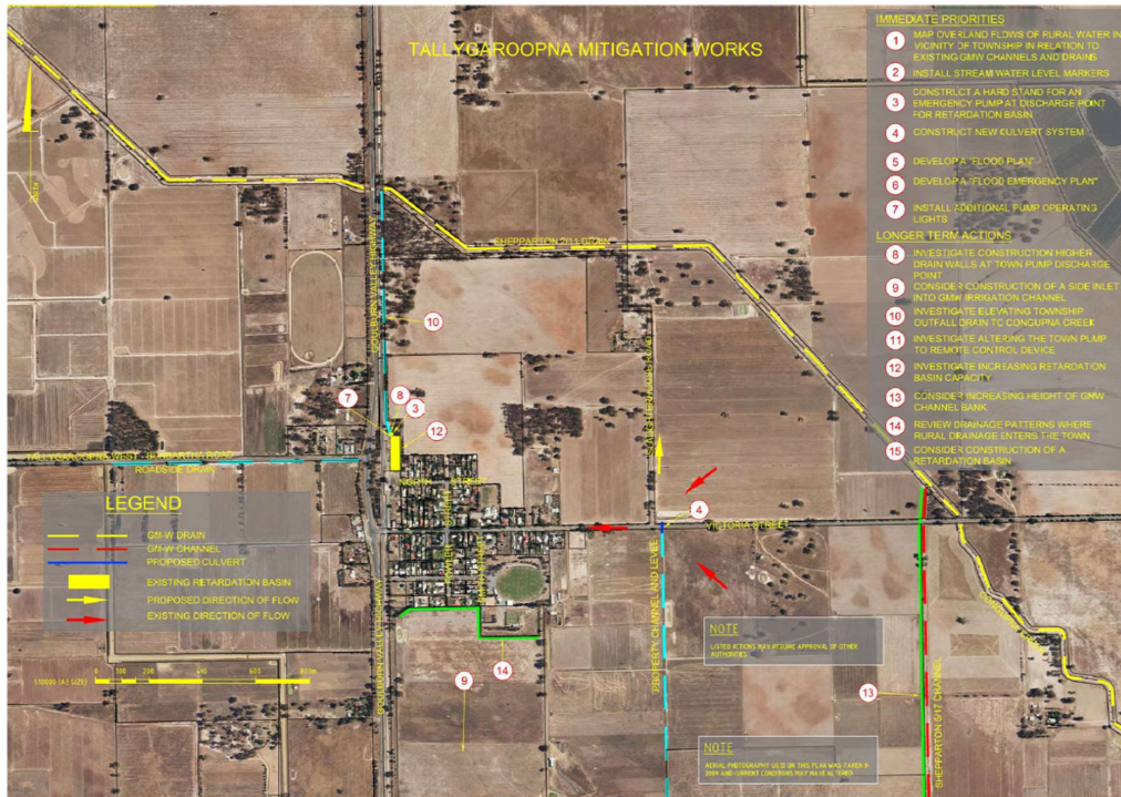
Figure 12 Tallygaroopna Drainage Improvement Plan – Post 2012 Event
