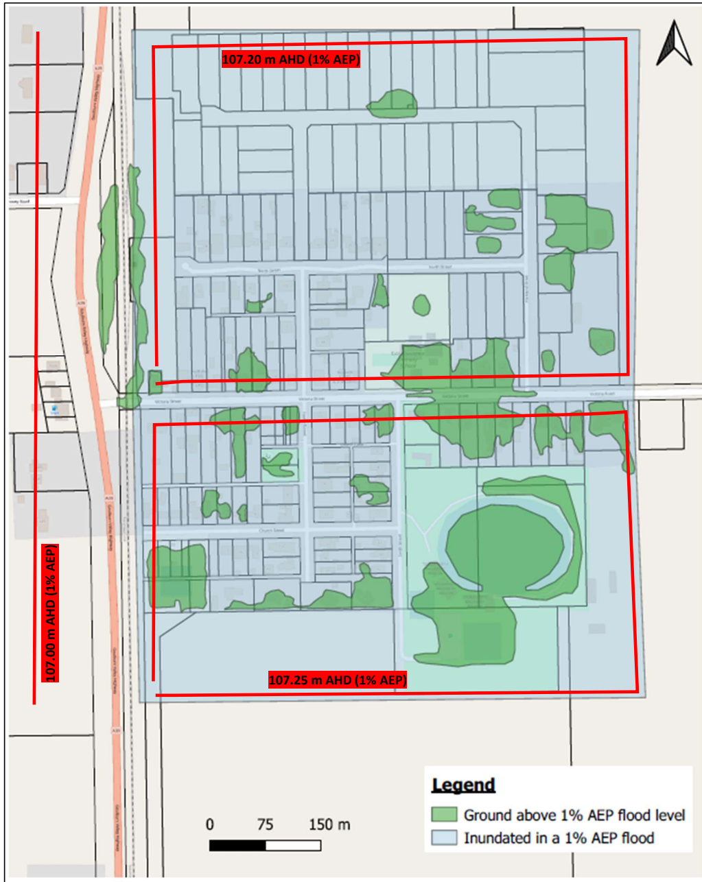
Figure 14 Tallygaroopna Township – 1% AEP Flood Extents and Heights
