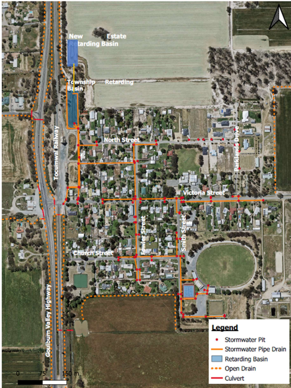
Figure 3 Stormwater Drainage Infrastructure at Tallygaroopna
