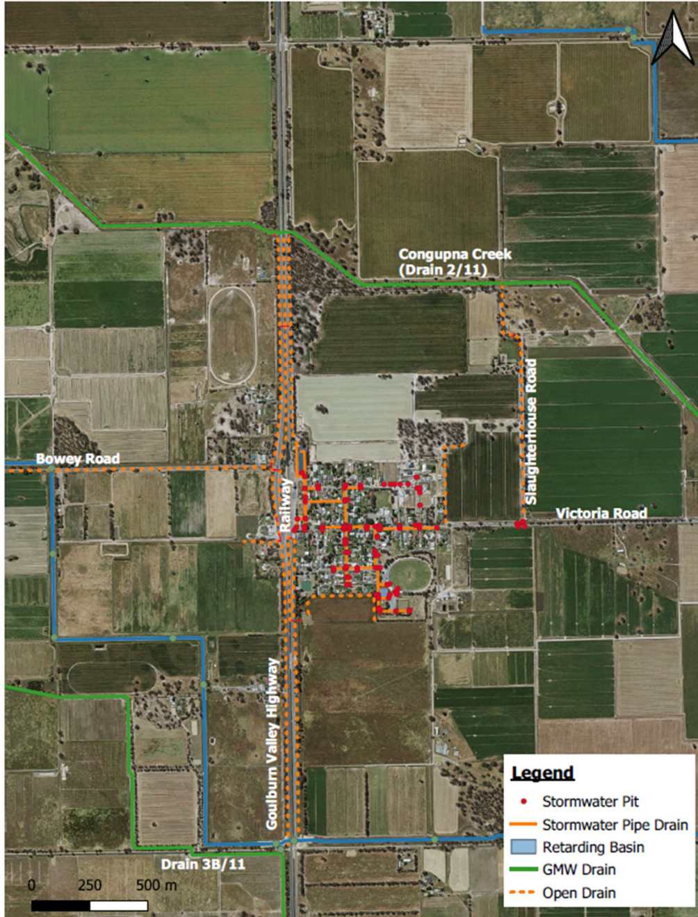
Figure 4 Drainage Infrastructure at Tallygaroopna
