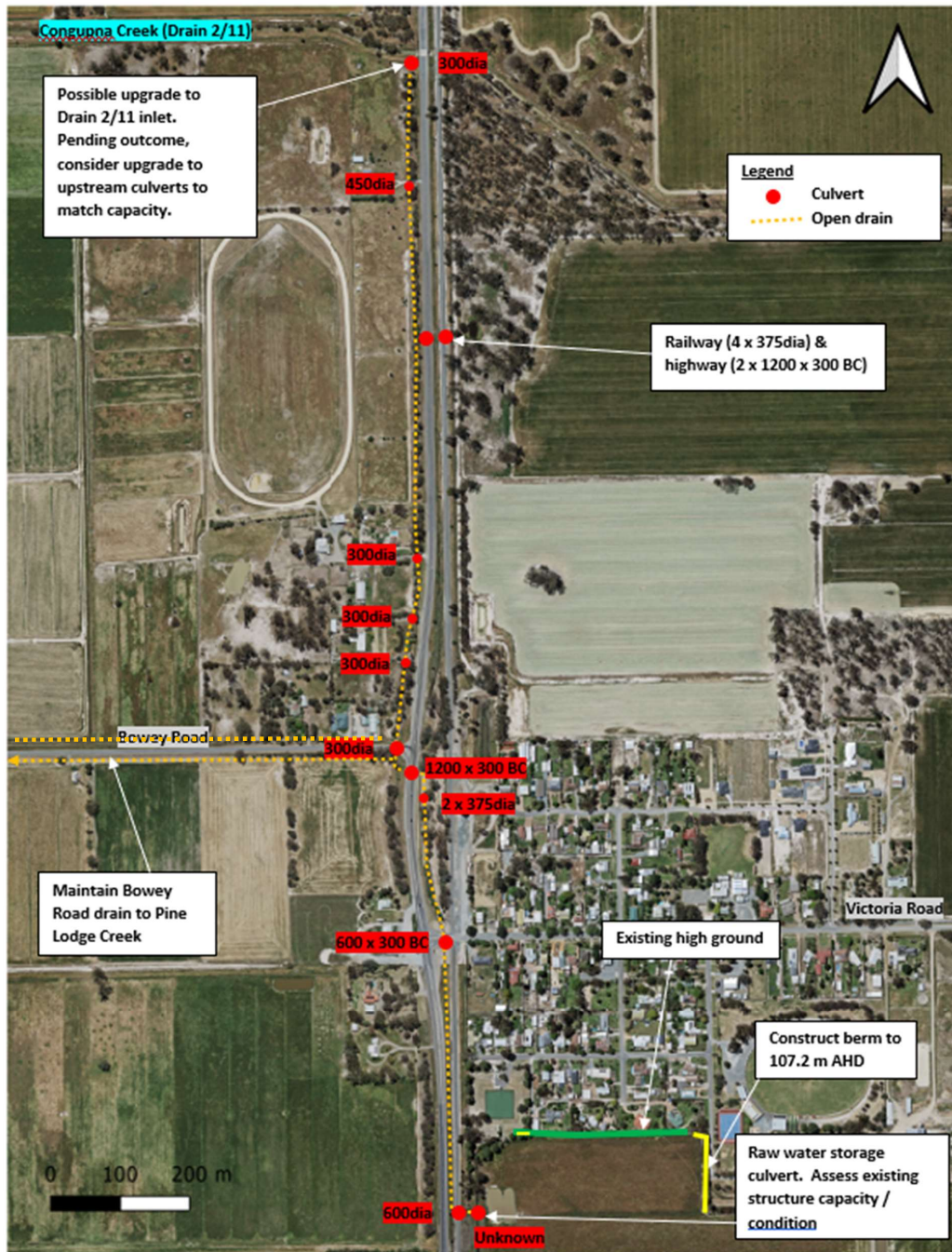
Figure 16 Diversion drain for south side rural runoff
