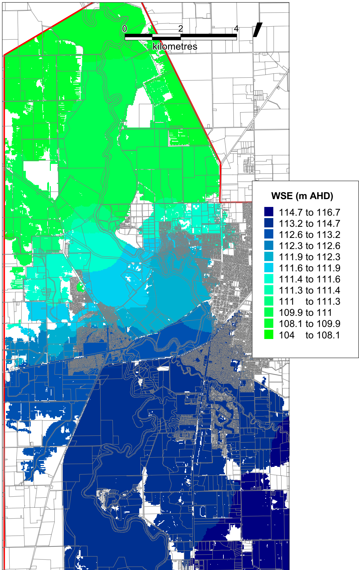
Figure 5 - 2005 Existing Conditions, 100 Year ARI Maximum Water Surface Elevation
