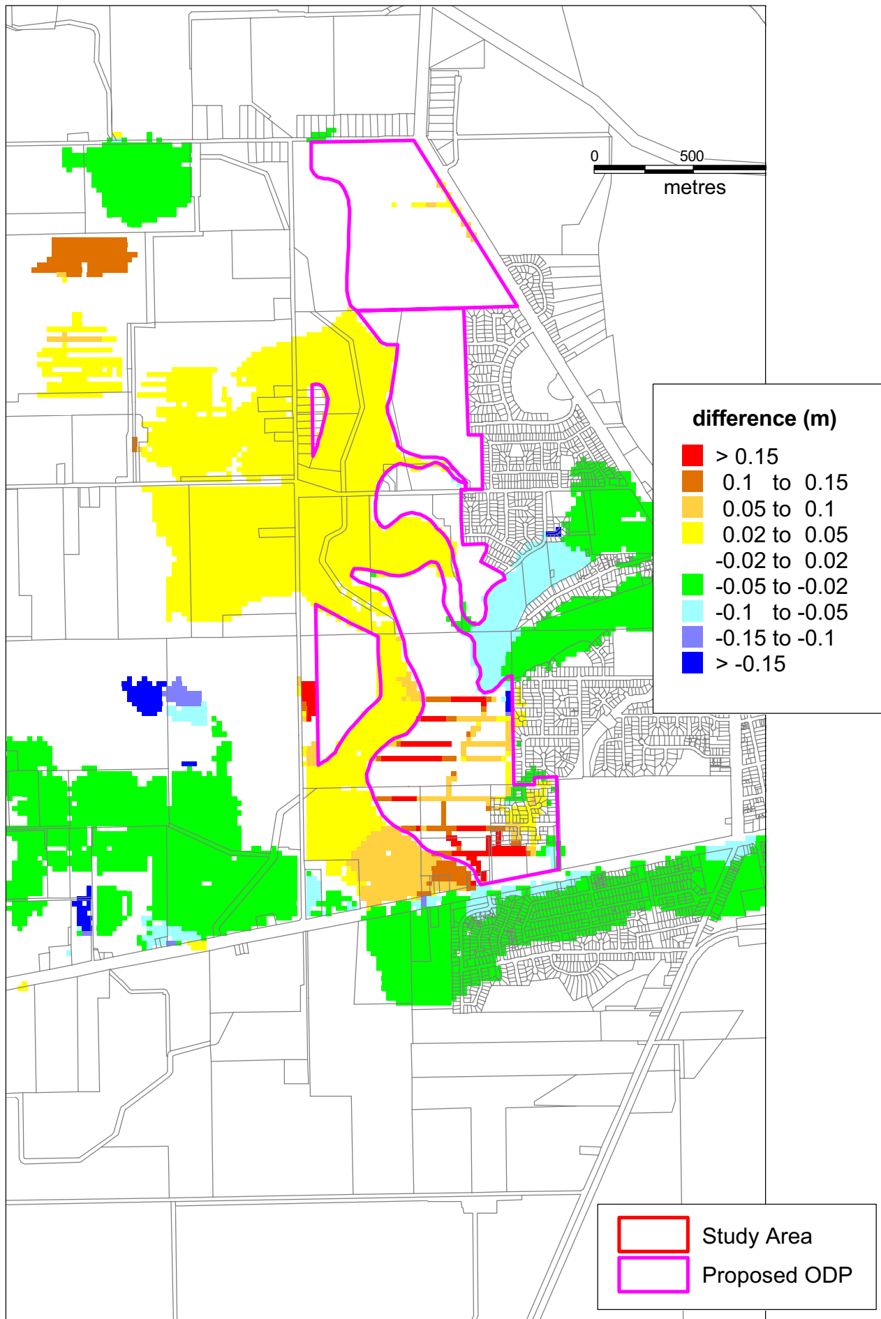
Figure 10 - WSE Difference - ODP Minus 2005 Conditions, 100 Year ARI Event
