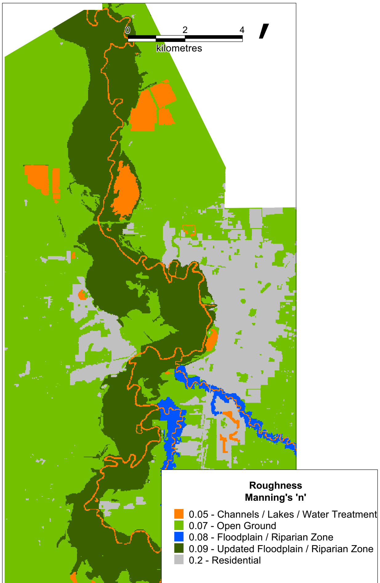
Figure 4 - Roughness, 2005 Conditions
