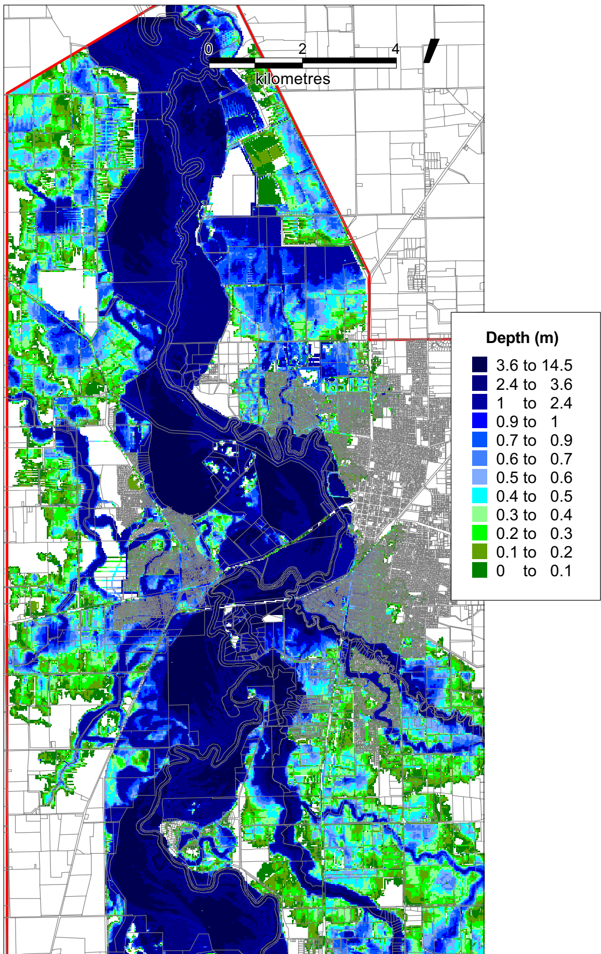
Figure 9 - 2005 Mooroopna ODP, 100 Year ARI Maximum Water Depth
