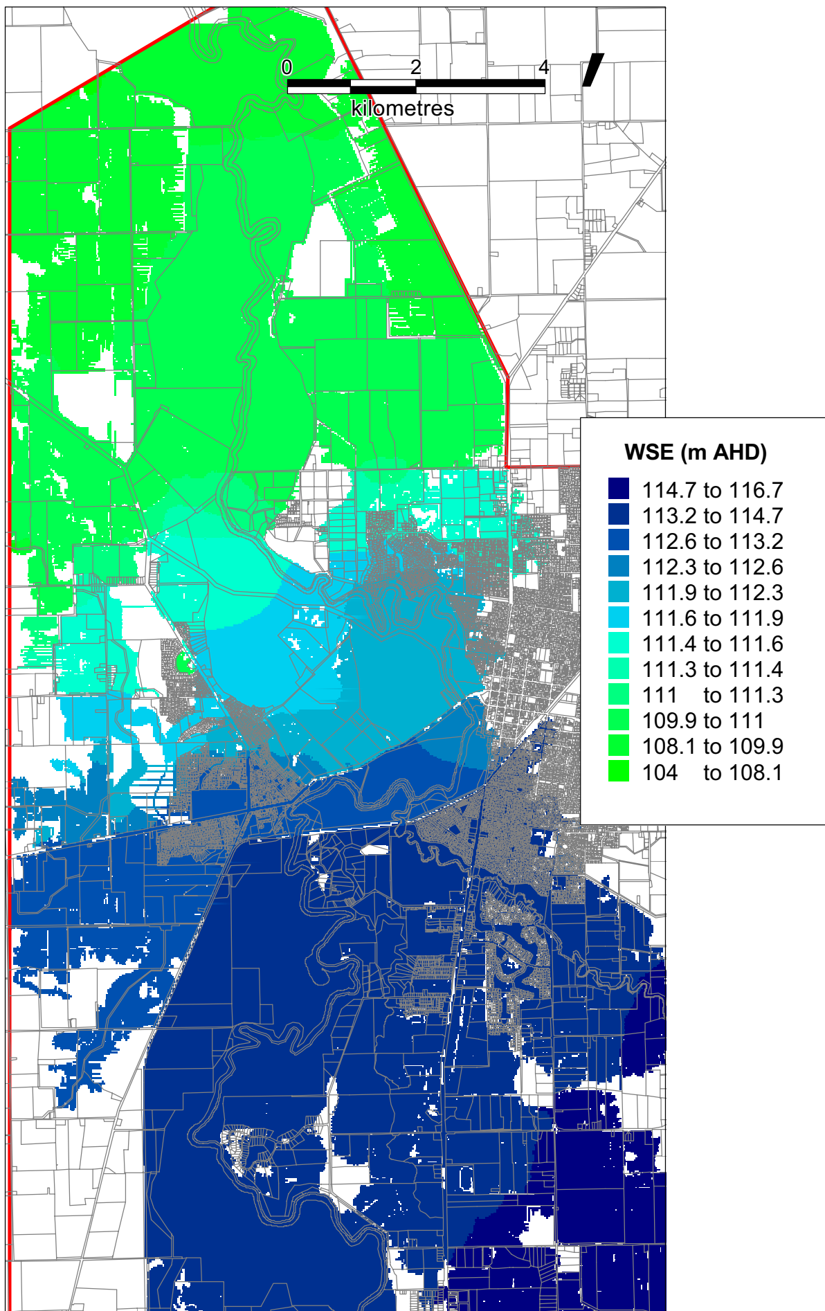
Figure 8 - 2005 Mooroopna ODP, 100 Year ARI Maximum Water Surface Elevation
