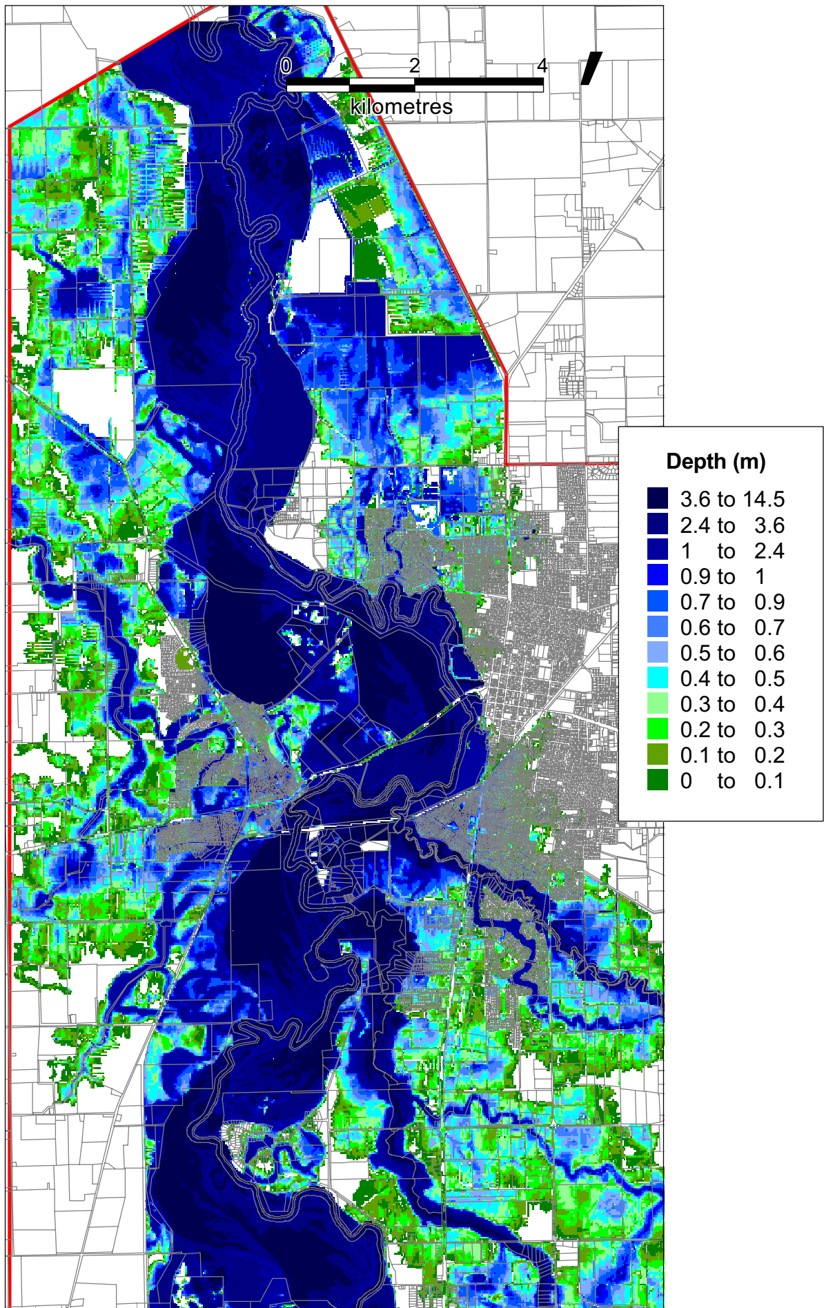
Figure 6 - 2005 Existing Conditions, 100 Year ARI Maximum Water Depth
